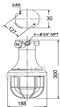
Ceiling mounting
